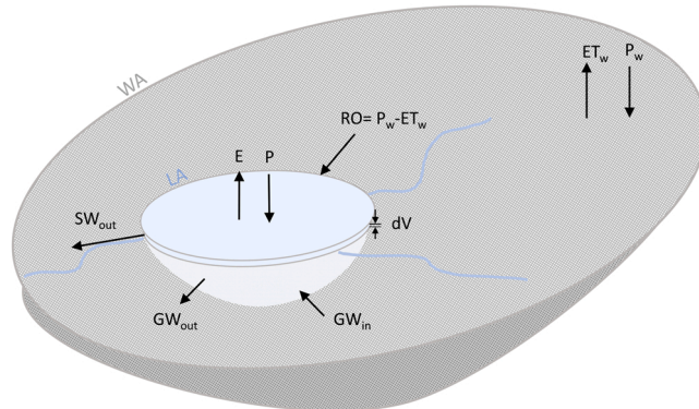
Fig. 2. Schematic of wetland-watershed system showing water balance fluxes. Note that P is precipitation on the lake, E is open water evaporation, RO is surface runoff, GW_{in} is groundwater inflow, GW_{out} is groundwater outflow, SW_{out} is surface outflow, and dV is change in volume. Note that P_w is precipitation on the watershed and ET_w is evapotranspiration from the watershed, where RO is approximated as P_w - ET_w . Wetland open water area ( LA ) and watershed area ( WA ) are determined based on areal delineations.
