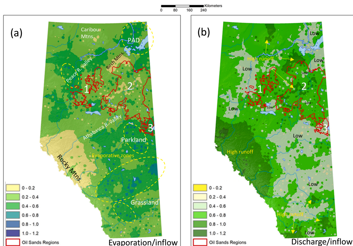
Fig. 6. Provincial maps showing distribution of complimentary water balance indicators based on isotope mass balance, (a) evaporation/inflow ( x ); (b) throughput i.e., total outflow/inflow ( \Sigma Q/I ). The three main oil sands regions are shown, including (1) Peace, (2) Athabasca, (3) Cold Lake. Evaporative zones are identified in Fig. 6a with yellow dashed ellipses; zones of high and low runoff ratios are labelled in Fig. 6b.
