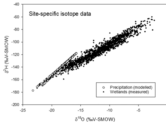
Fig. 3. Dual isotope plot showing measured isotopic composition of wetlands for Alberta, 2009–2018 (solid circles) compared to mean annual precipitation (open circles). Note that modelled mean annual precipitation is based on Delavau et al. (2015) and closely resembles the CMWL.
