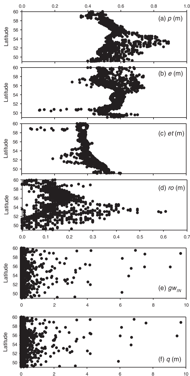
Fig. 5. Latitudinal variations in water balance fluxes, including (a) precipitation, (b) evaporation from open water, (c) evapotranspiration, (d) watershed runoff, estimated as P-ET using Eq. (4), (e) calculated groundwater inflow, and (f) total outflows including surface and groundwater outflows.
