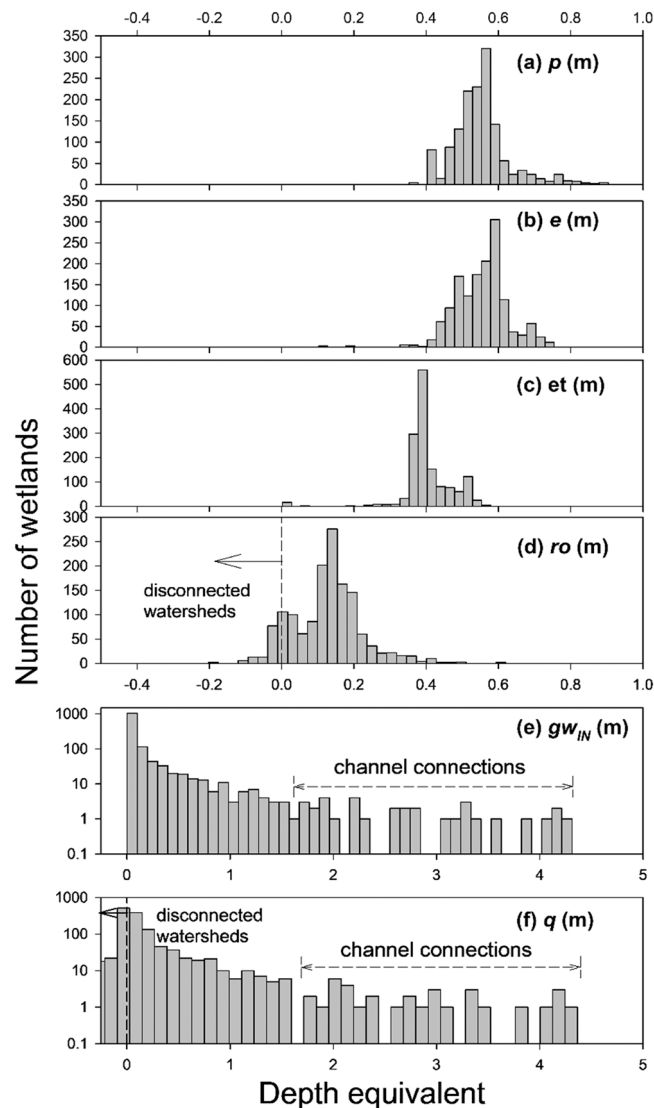
Fig. 4. Histograms showing depth-equivalent water balance fluxes for open water wetlands across the province, including (a) precipitation, (b) evaporation from open water, (c) evapotranspiration, (d) watershed runoff, (e) groundwater inflow to wetlands (normalized to watershed area), and (f) total outflows (normalized to watershed area). Negative runoff and negative total outflows are identified for disconnected watersheds. Unrealistic inflows/outflows (and exaggerated positive skews) shown in (e) and (f) at ~30 sites are attributed to connection/interaction with stream channels.
