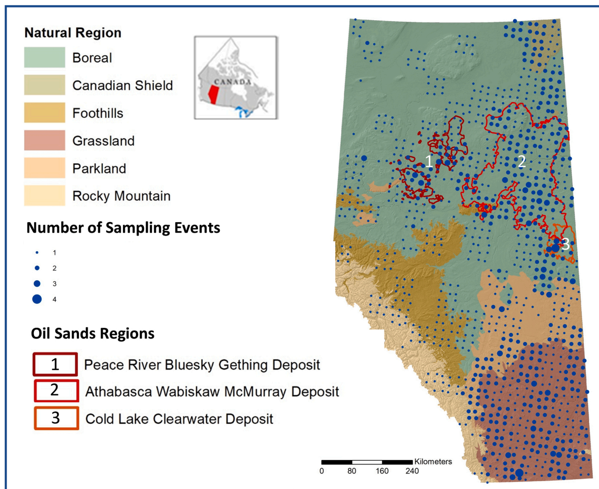
Fig. 1. Map of Alberta, Canada showing location of ABMI open water wetlands sampled between 1 and 4 times during the field program. Natural regions and the three main oil sands regions of Alberta are also shown.
