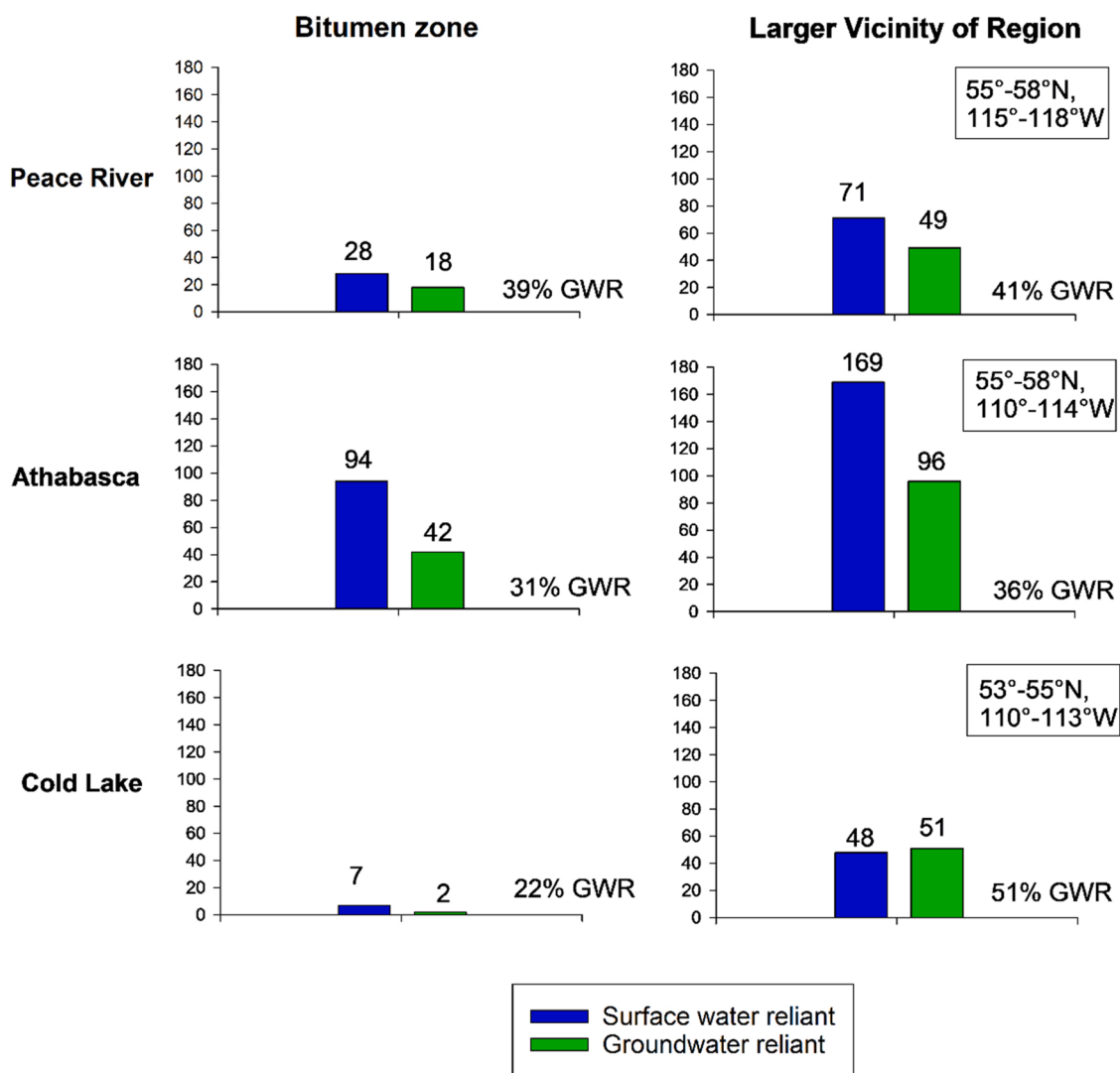
Fig. 8. Counts of surface water reliant and groundwater reliant wetlands in the three oil sands regions based on isotope mass balance. Oil sands bitumen extent for each region is shown in Fig. 1; latitude-longitude ranges are provided.
