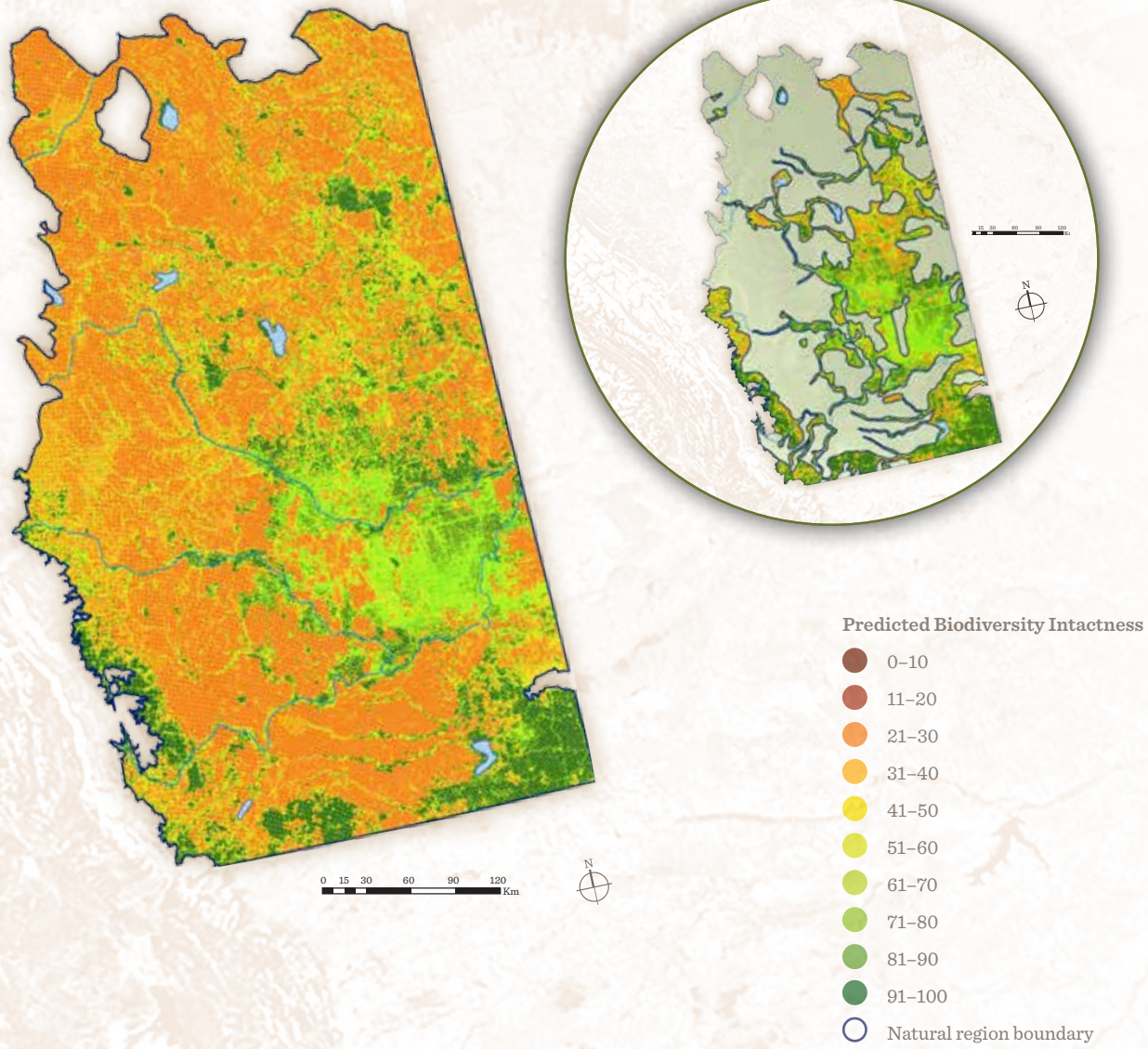
FIGURE 08. Average predicted intactness in the Prairie Region (left map) and inside the High Value Landscape (right map). Dark red and orange quarter sections are predicted to have the lowest average biodiversity intactness while dark green quarter sections have the highest average intactness.
